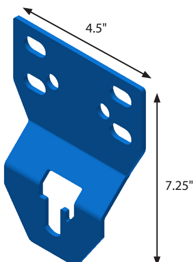
545CIR DWG #434
