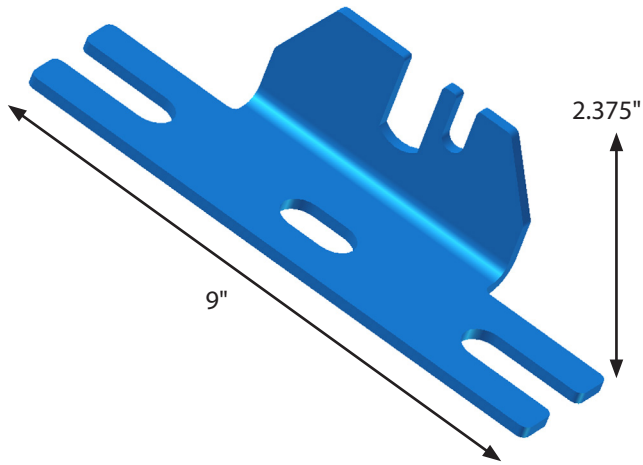
915BPS DWG #642
