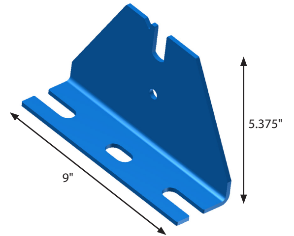
945BPS DWG #179
