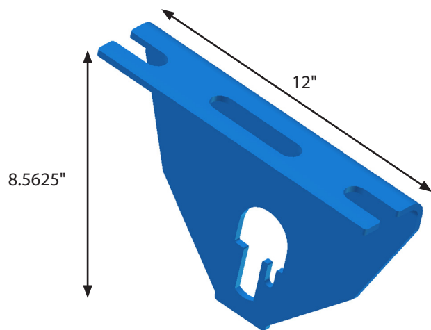
1270BPSR DWG #458
