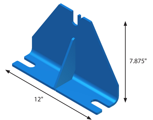
1270BPS DWG #2797-B
